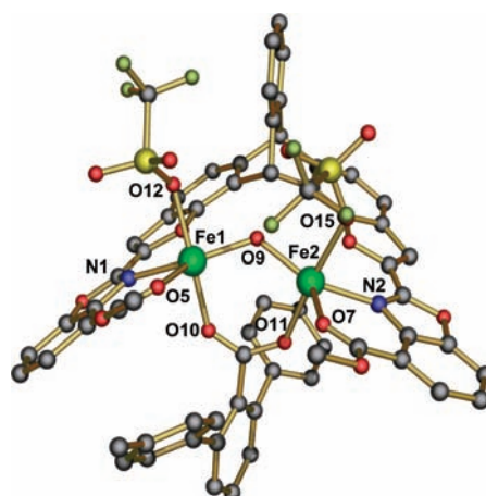
Figure 3. X-ray crystal structure of complex [Fe 2 L1(μ-OH)(μ-O 2 CAr Tol )(OTf) 2 ]. Selected bond distances (Å) and angles (deg): Fe(1)–Fe(2) = 3.443; Fe(1)–N(1) = 2.139(6); Fe(1)–O(5) = 2.114(6); Fe(1)–O(9) = 1.949(5); Fe(1)–O(10) = 2.071(5); Fe(1)–O(12) = 2.147(5); Fe(2)–N(2) = 2.116(6); Fe(2)–O(7) = 2.107(5); Fe(2)–O(9) = 1.944(5); Fe(2)–O(11) = 2.059(5); Fe(2)–O(15) = 2.207(5); Fe(1)–O(9)–Fe(2) = 124.4(3); N(1)–Fe(1)–O(9) = 154.1(2); N(2)–Fe(2)–O(9) = 149.6(2).
