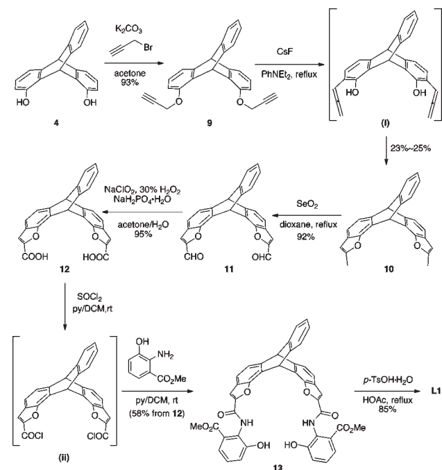
Scheme 2. Synthesis of Ligand L1 from 4
